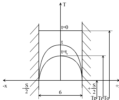
Fig.2.Cooling material plastic in the moulds:
