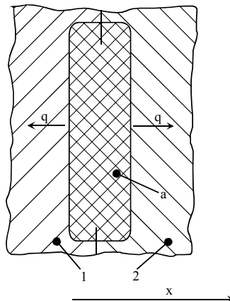
Fig.1. The thermal transfer in case of the injection pieces in mould: 1,2-forming plates; a- injected pieces; q-thermal high tide unitary on x direction. They are introduced the following simplifying hypothesis:
