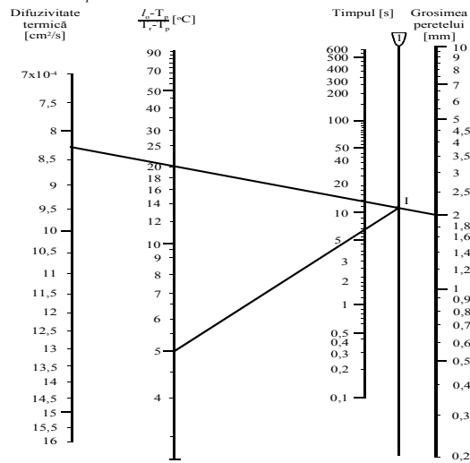
Fig.3. Nomograma for determining the cooling time in case of injected piece plate.
