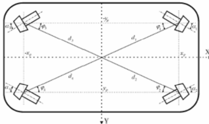
Fig. 3. Layout of thrusters in the subsystem responsible for the horizontal motion.
