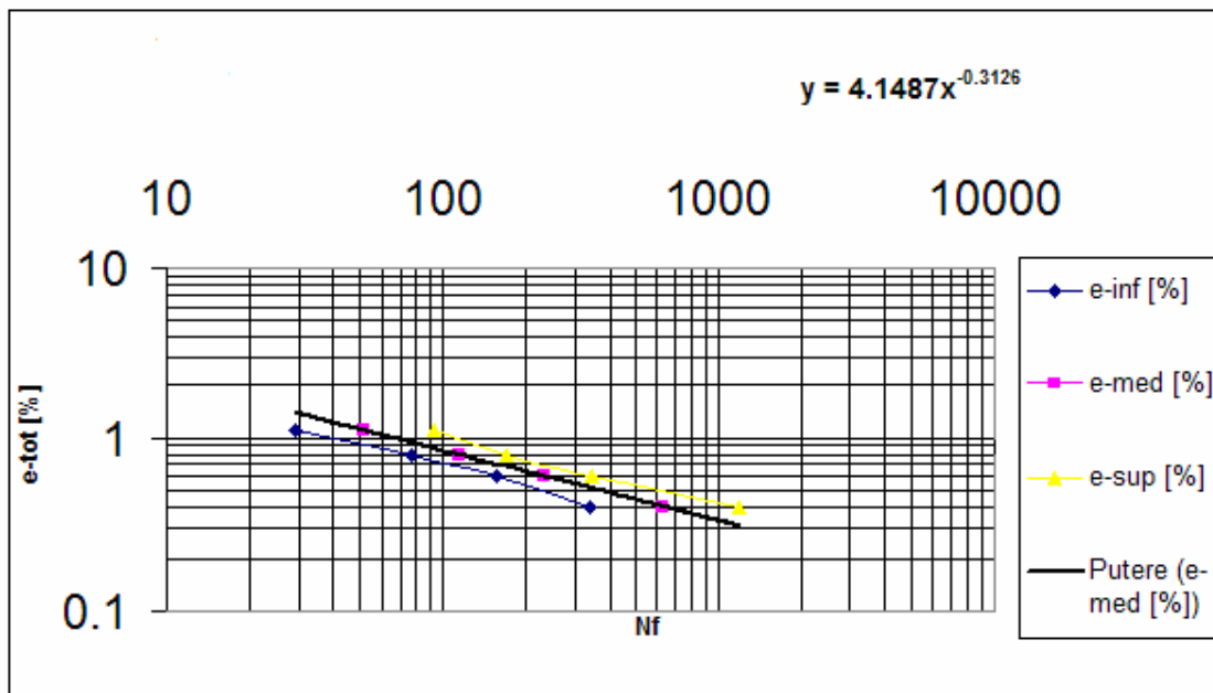
Fig.3. Manson-Coffin Equation from 16Mo5.3b steel, the thermomechanical fatigue tests are conducted in temperature range 60^\circ \leftrightarrow 540^\circ\text{C} , with 3600 second soaking period at maximum temperature of 540^\circ\text{C} .
